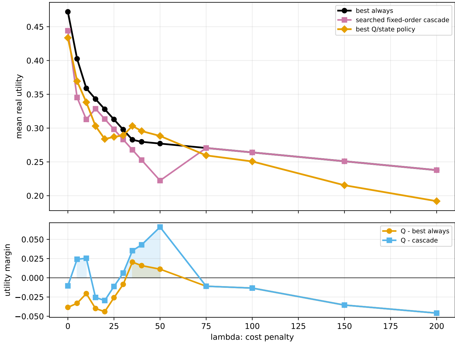
Fair fixed-cost Q/state policy vs cascade (full lambda range)
