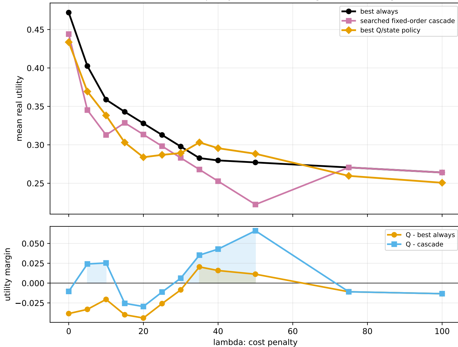
Fair fixed-cost Q/state policy vs cascade (budget-sensitive region)
