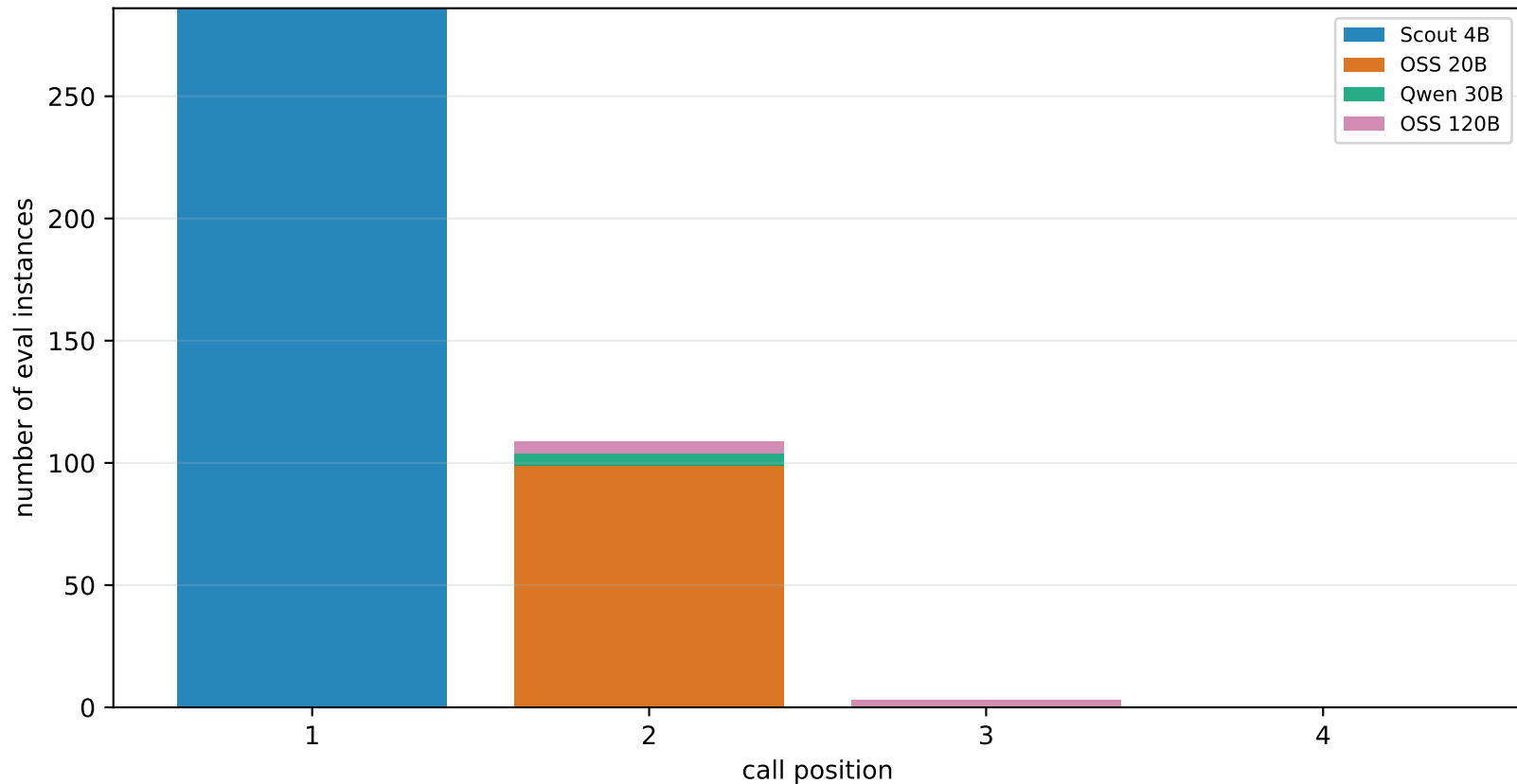
Q forced-scout chain: routes called by step, lambda=100
