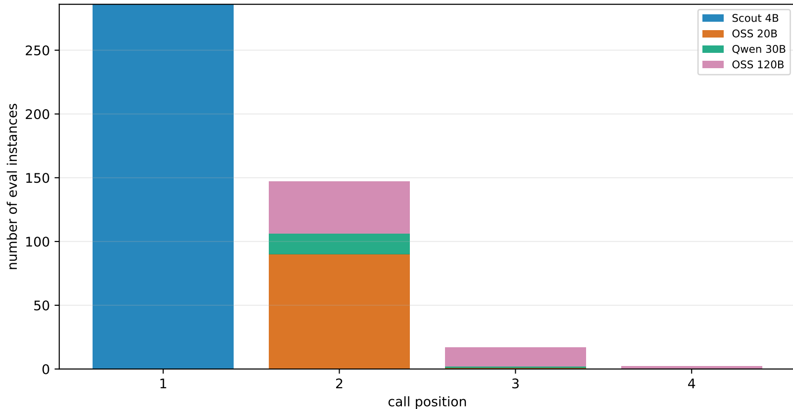
Q forced-scout chain: routes called by step, lambda=25
