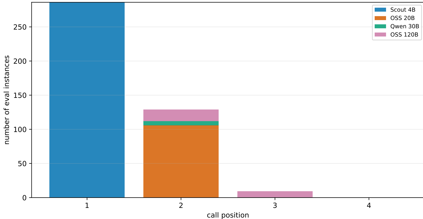
Q forced-scout chain: routes called by step, lambda=50
