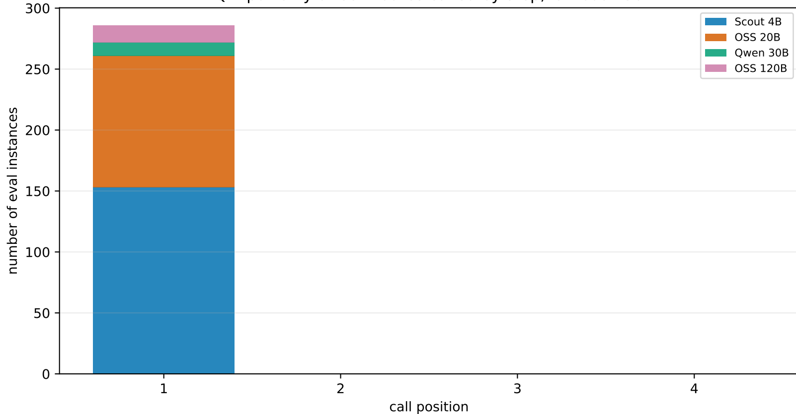
Q input-only direct: routes called by step, lambda=50
