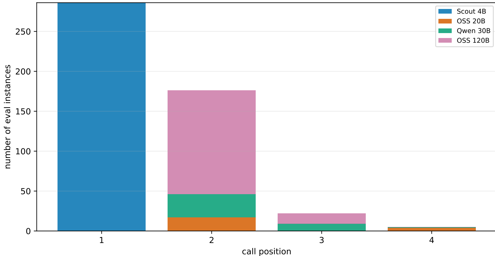
Q forced-scout chain: routes called by step, lambda=5
