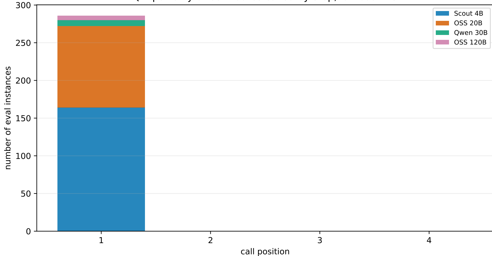
Q input-only direct: routes called by step, lambda=75
