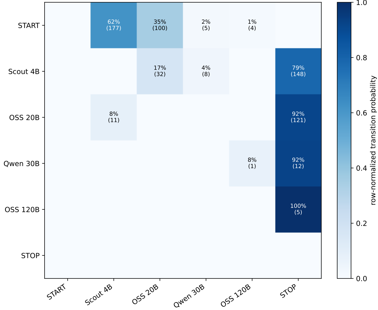
Q flexible chain: transition probabilities, lambda=100
