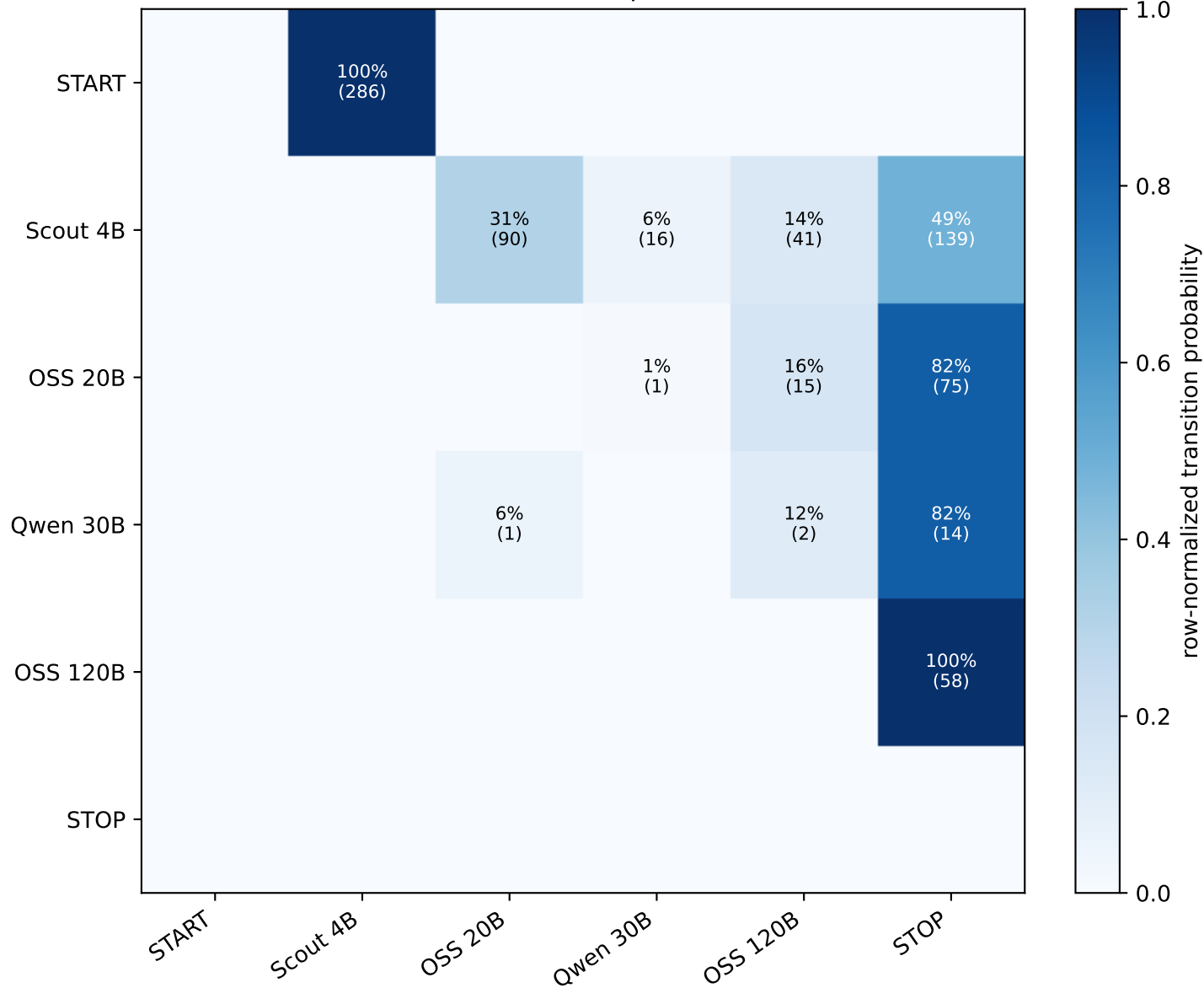
Q forced-scout chain: transition probabilities, lambda=25
