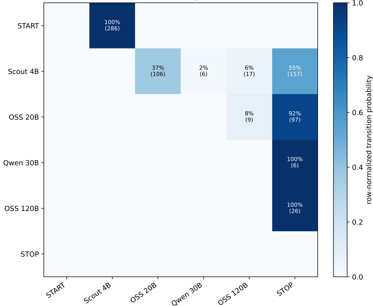
Q forced-scout chain: transition probabilities, lambda=50
