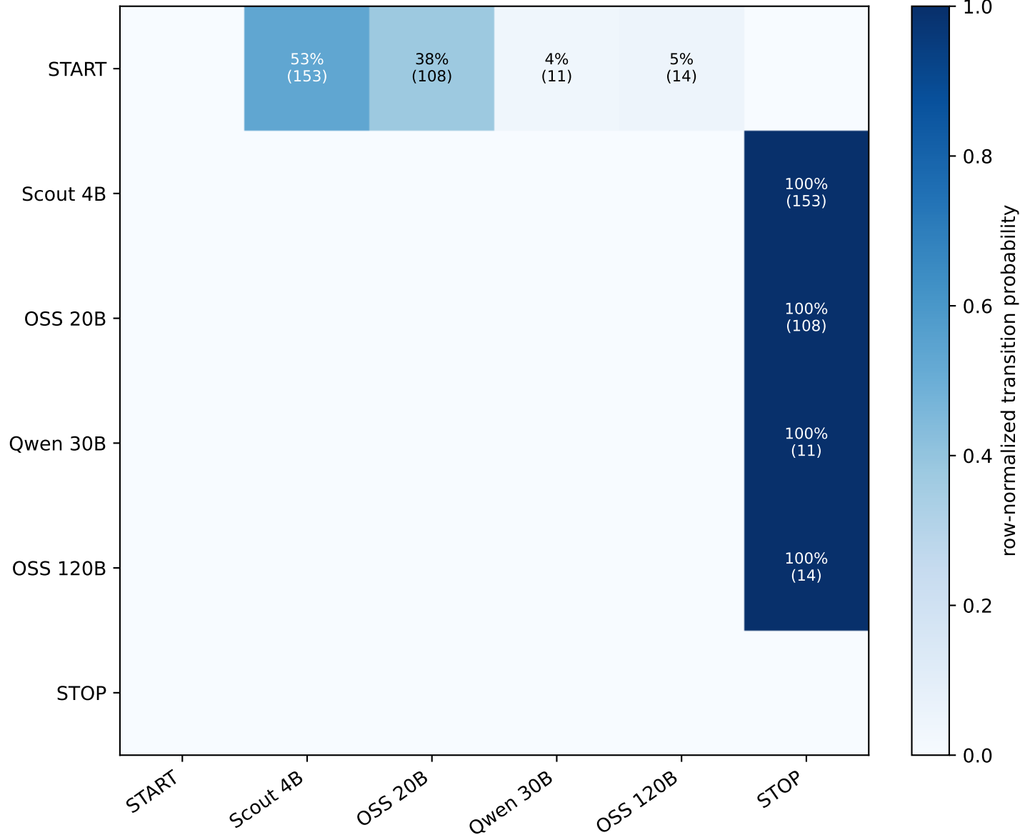
Q input-only direct: transition probabilities, lambda=50
