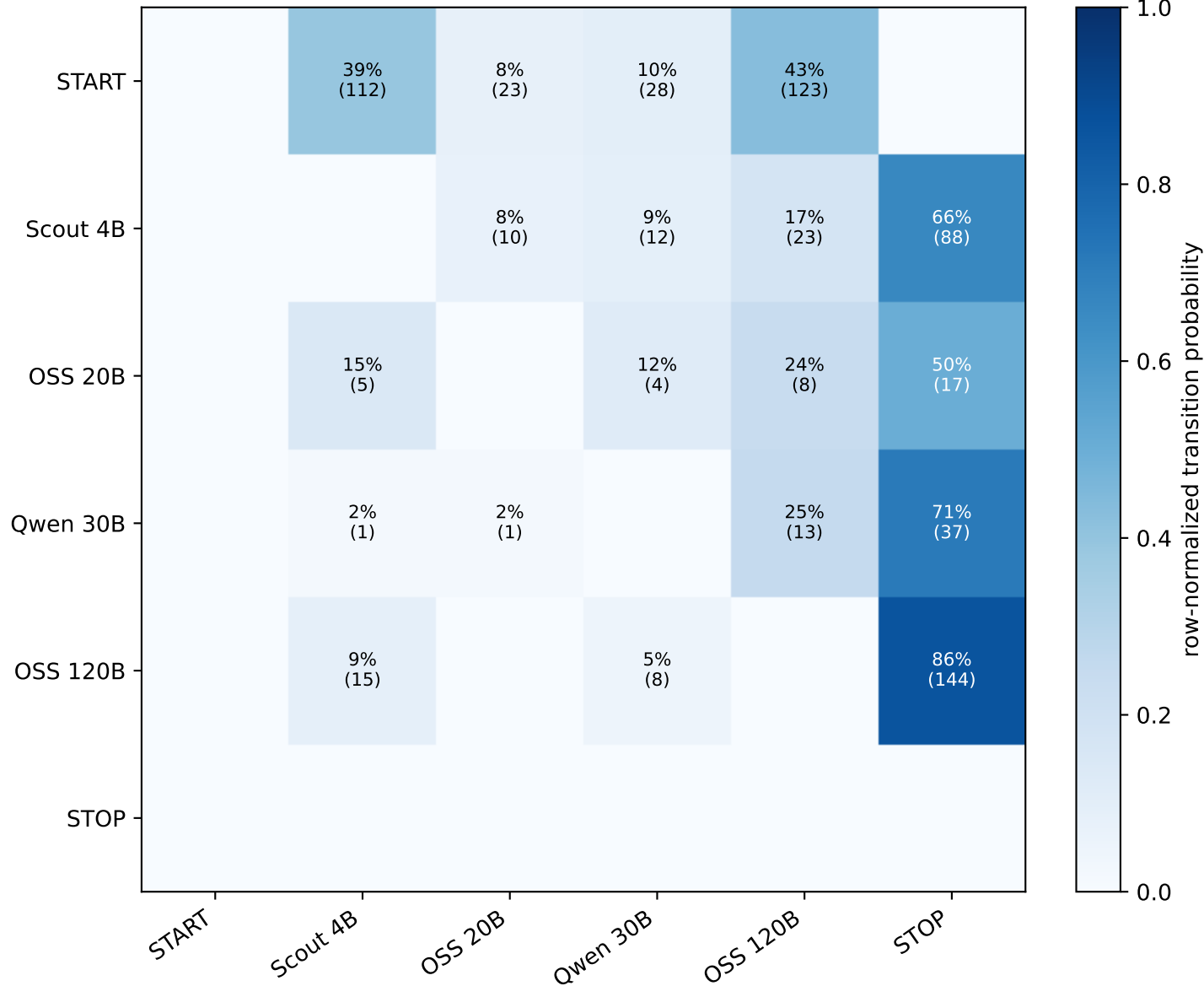
Q flexible chain: transition probabilities, lambda=5
