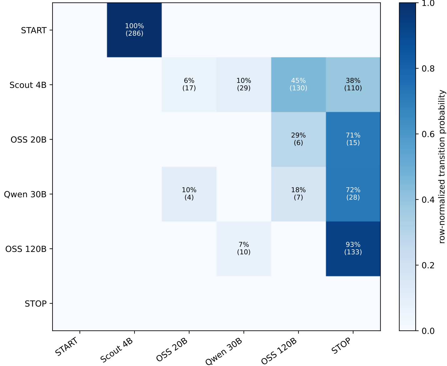
Q forced-scout chain: transition probabilities, lambda=5
