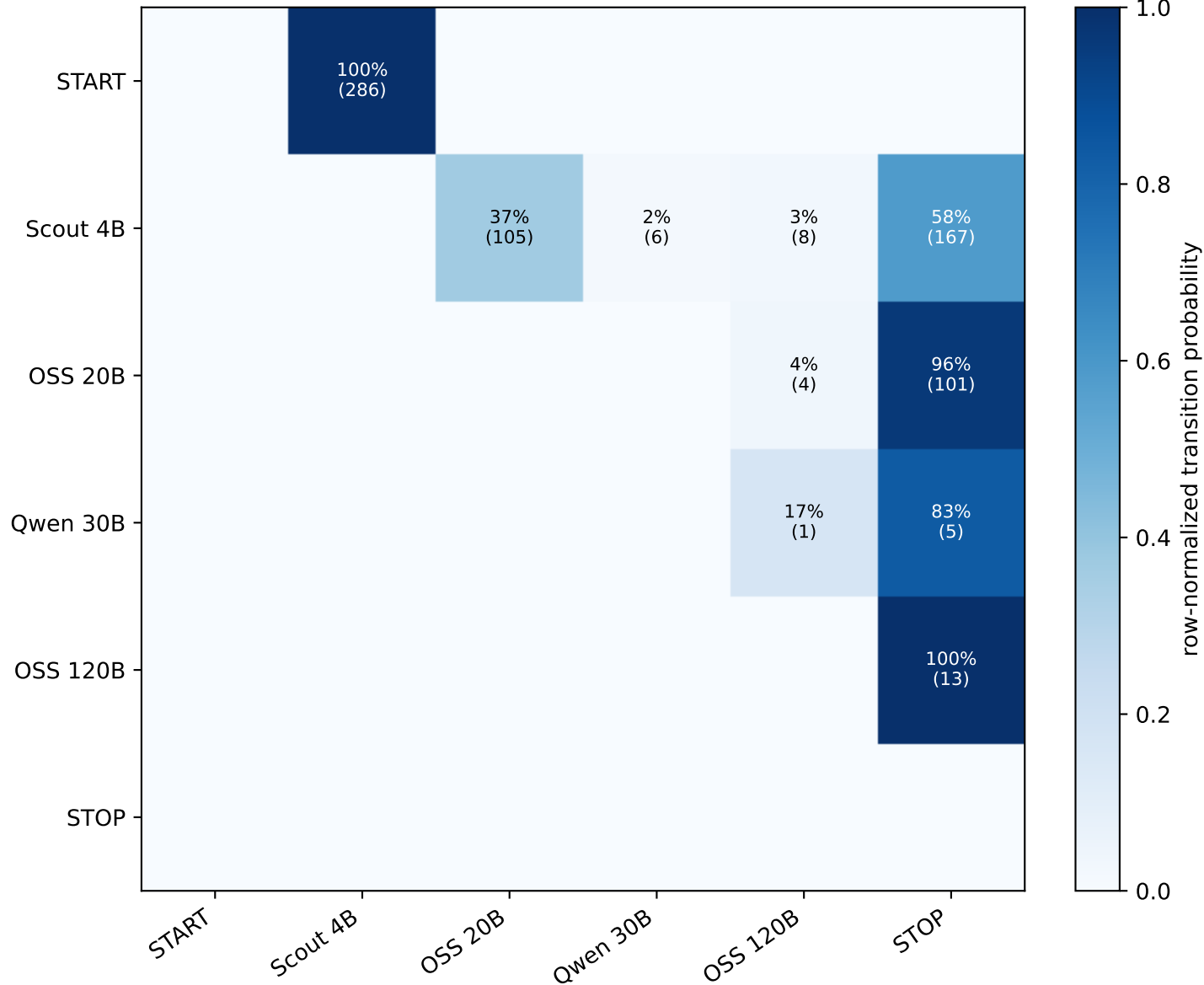
Q forced-scout chain: transition probabilities, lambda=75
