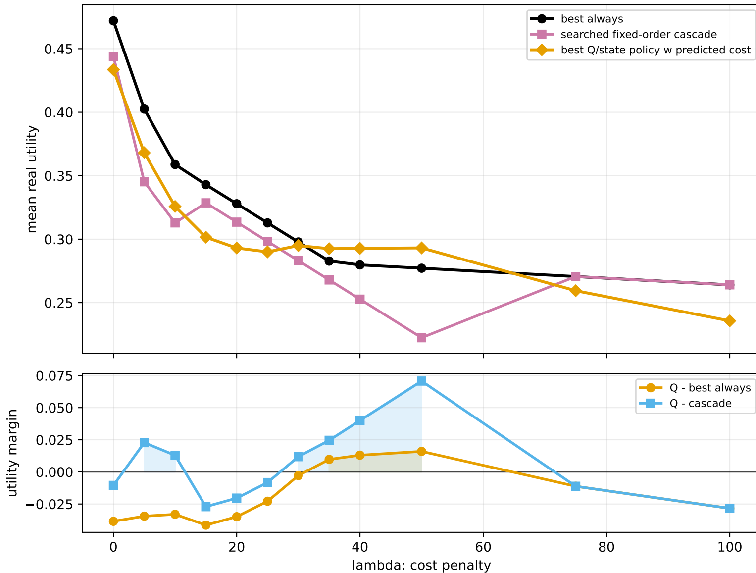
Predicted-cost Q/state policy vs cascade (budget-sensitive region)
