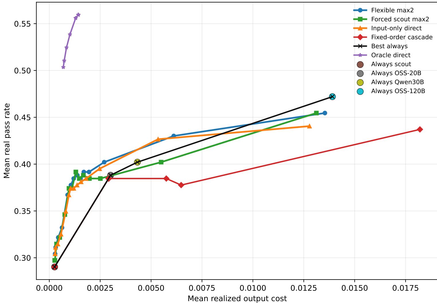
Real pass rate vs realized output cost
