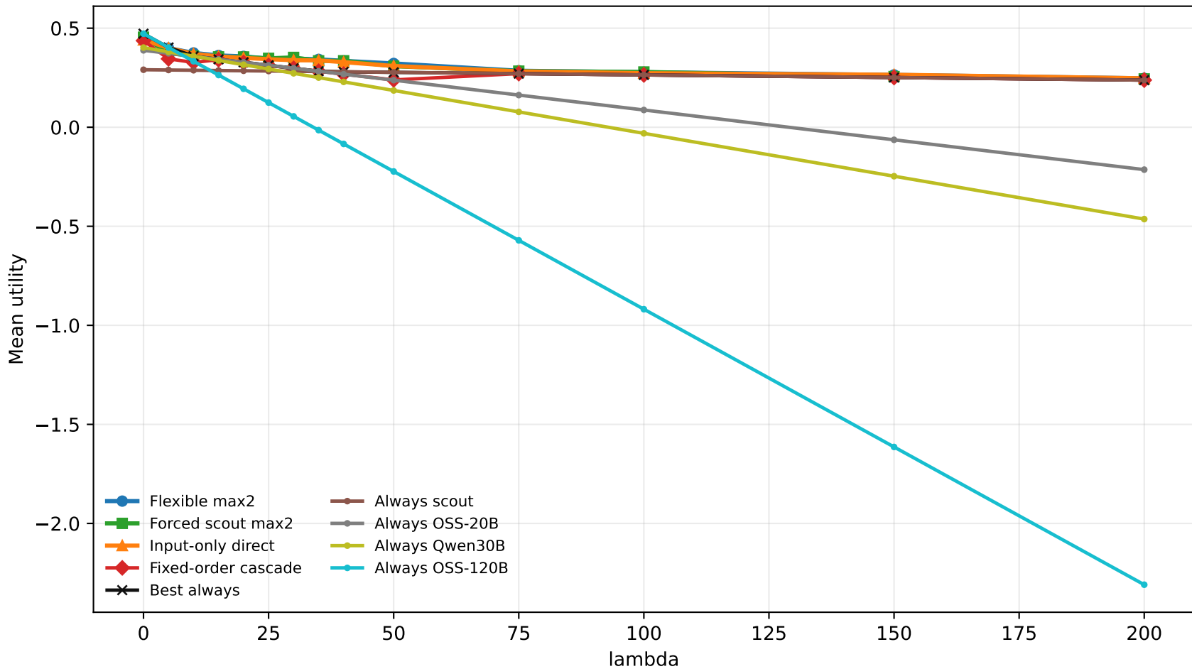
Utility vs lambda with individual always baselines
