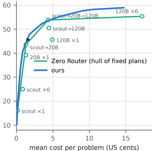
TACO (seed 0): 22% cheaper than the Zero Router at gpt-oss-120b's accuracy (arrow)
