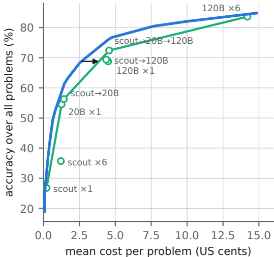
LiveCodeBench (seed 0): 31% cheaper than the Zero Router at gpt-oss-120b's accuracy (arrow)
