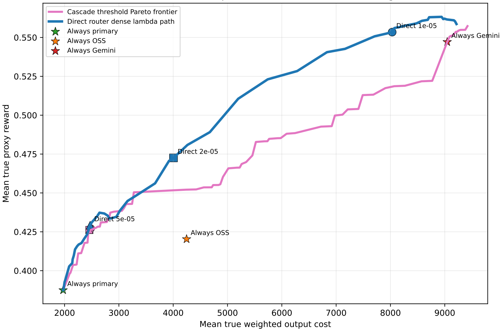
Dense direct-router lambda path vs cascade frontier (cost weights 1/3/20)
