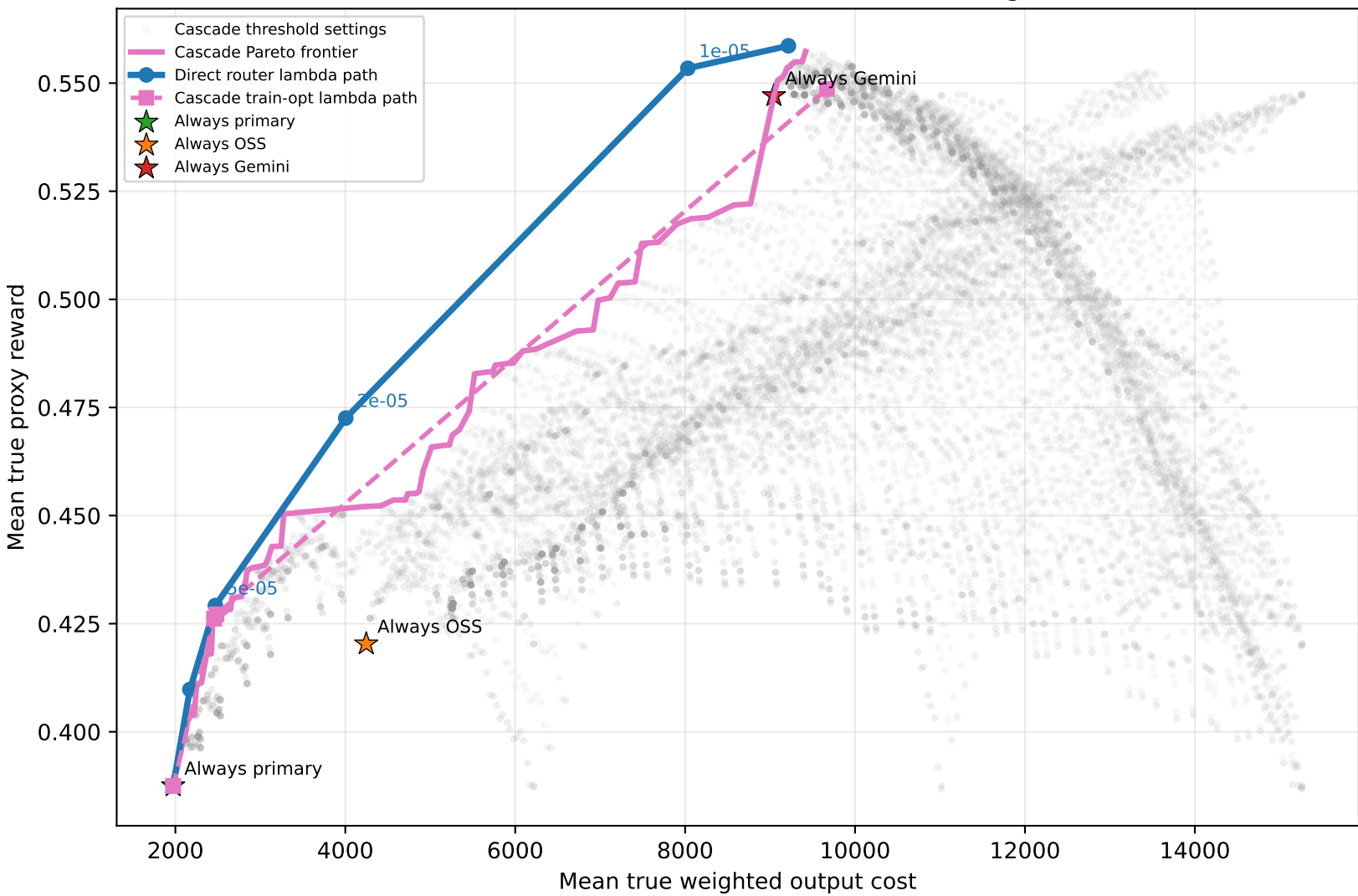
Cascade threshold frontier vs direct router (cost weights 1/3/20)
