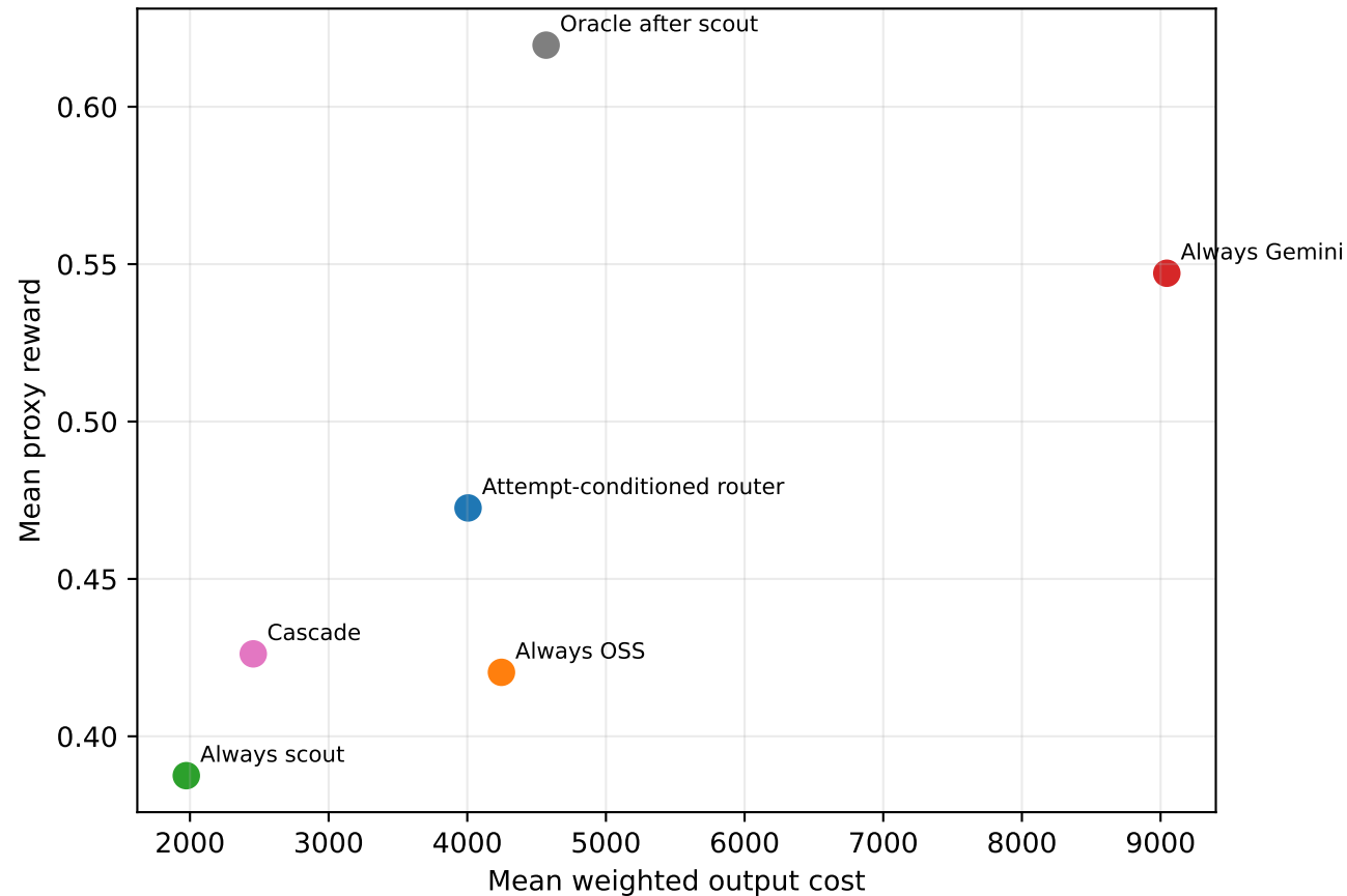
Reward/cost at \lambda=2e-5
