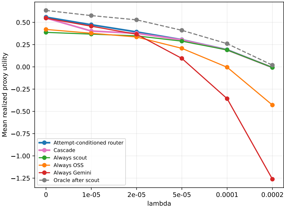
Utility across cost multipliers
