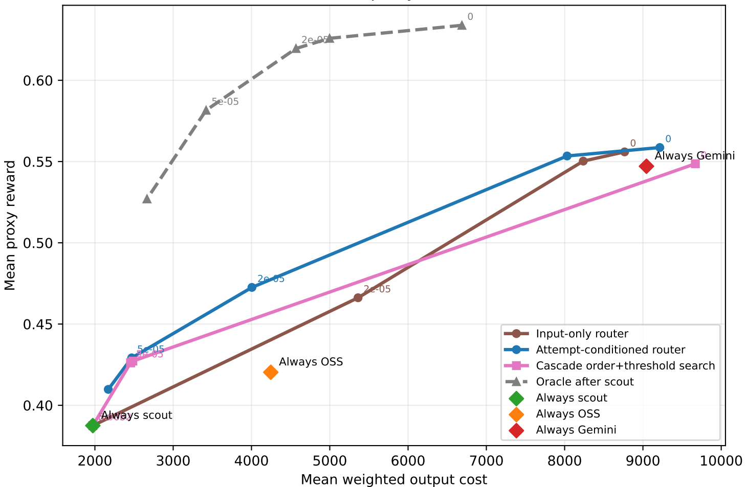
SWE-Bench Verified proxy reward/cost frontier
