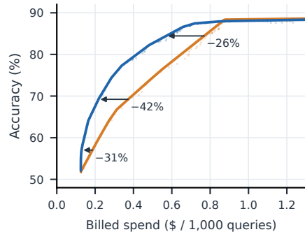
LiveCodeBench (341 test)
