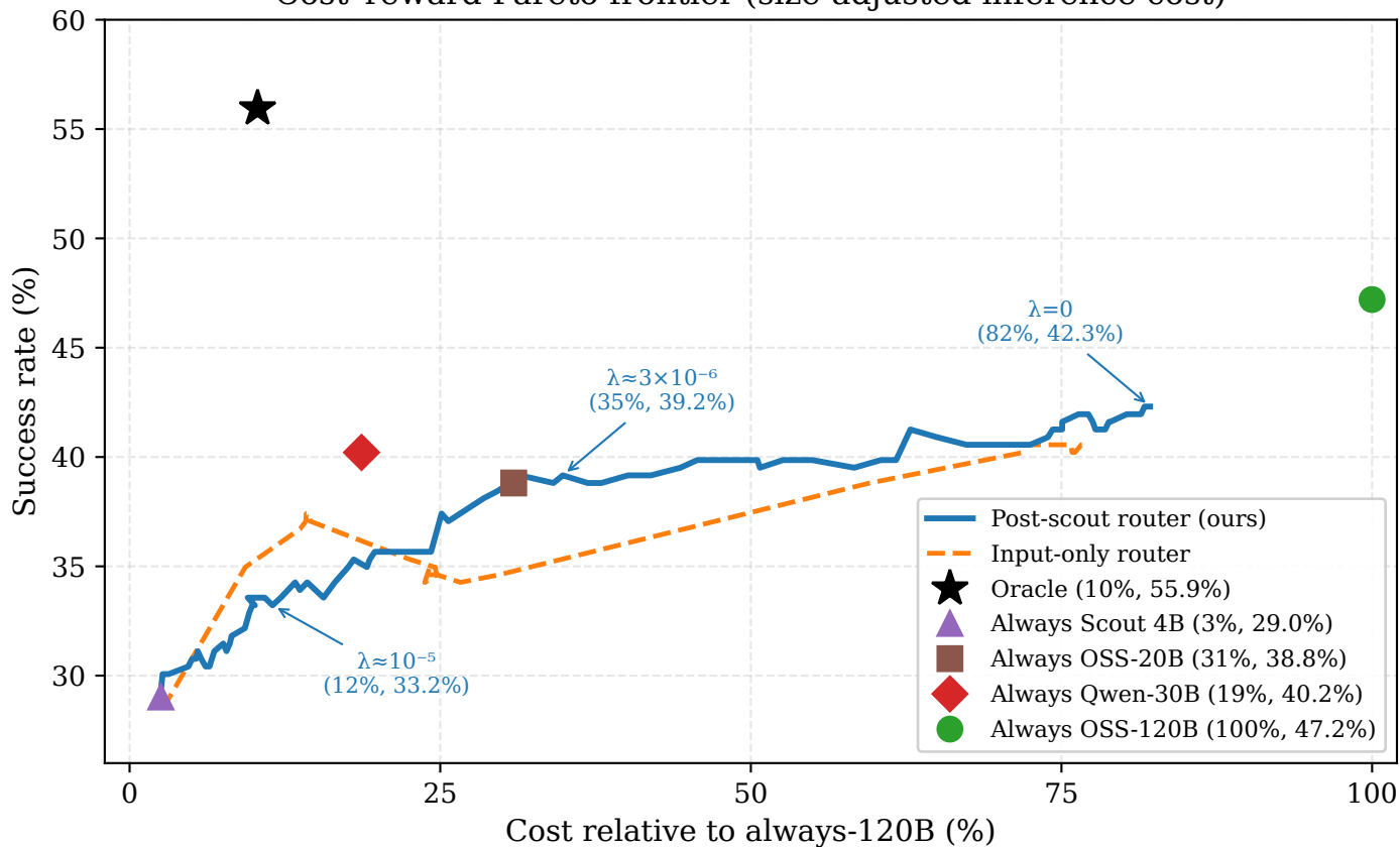
Cost-reward Pareto frontier (size-adjusted inference cost)
