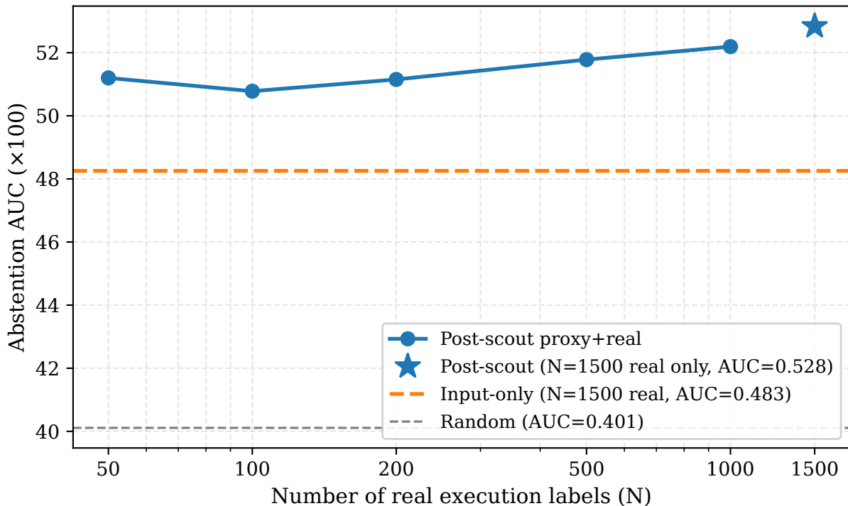
Sample efficiency: proxy pre-training + real fine-tuning
