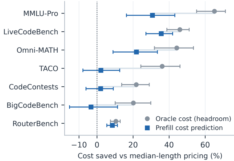
Figure 1. Available savings can remain uncaptured. Oracle and predicted costs replace median output length with success predictions held fixed. Whiskers are paired 95% problem-bootstrap intervals. Oracle headroom alone does not establish a learnable routing signal.
