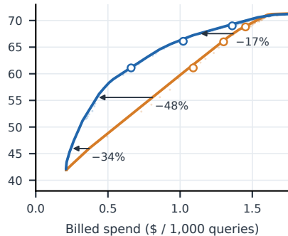
Omni-MATH (1,000 test)
