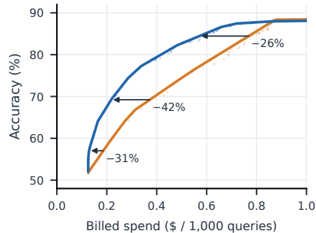
LiveCodeBench (341 test)
