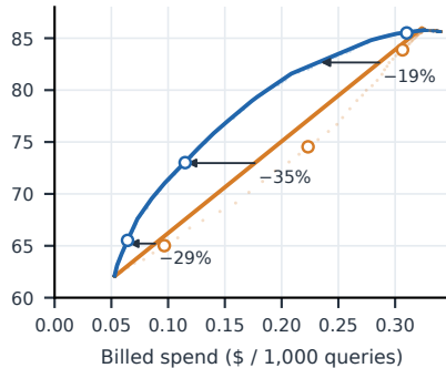
MMLU-Pro (6,500 test)
