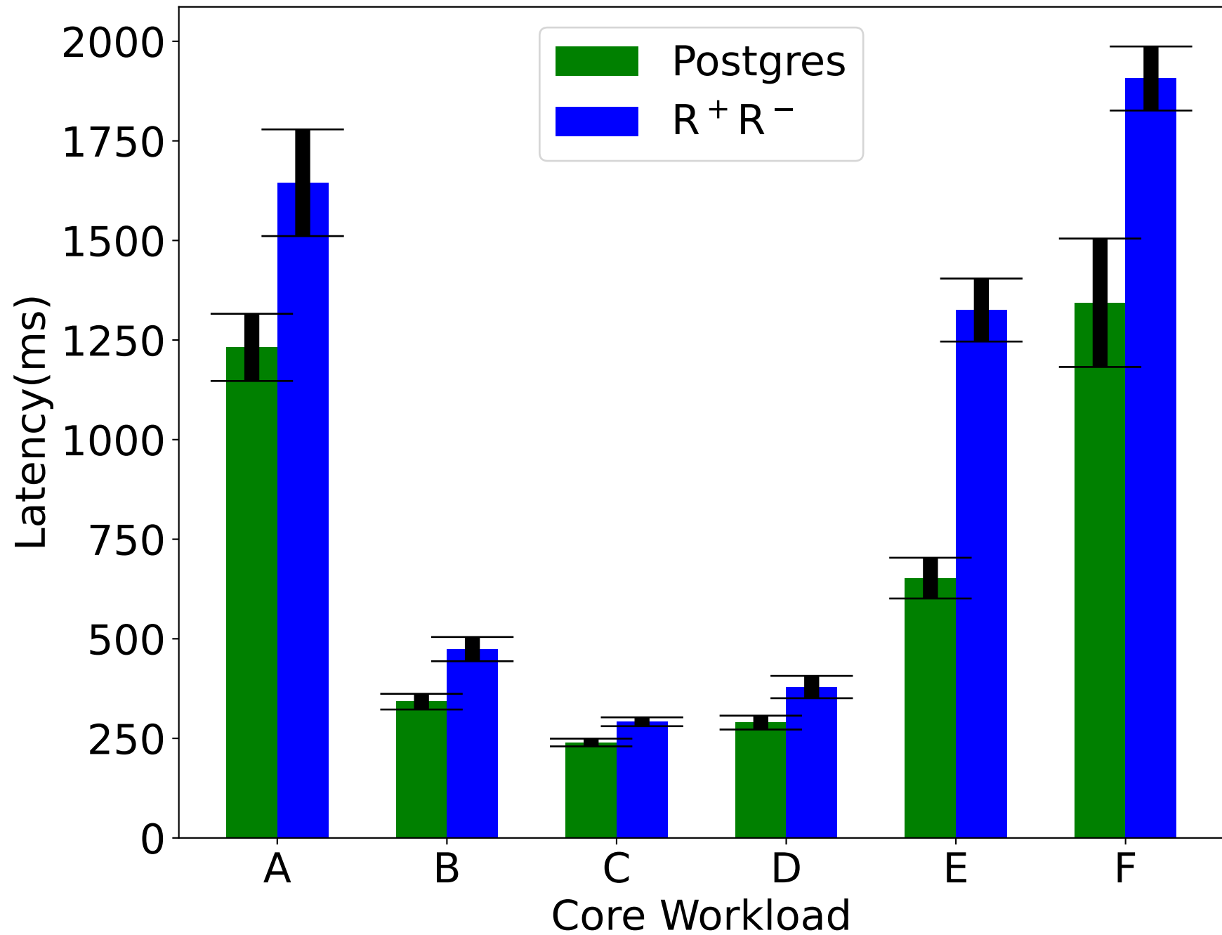
YCSB Benchmark 1M Rows
