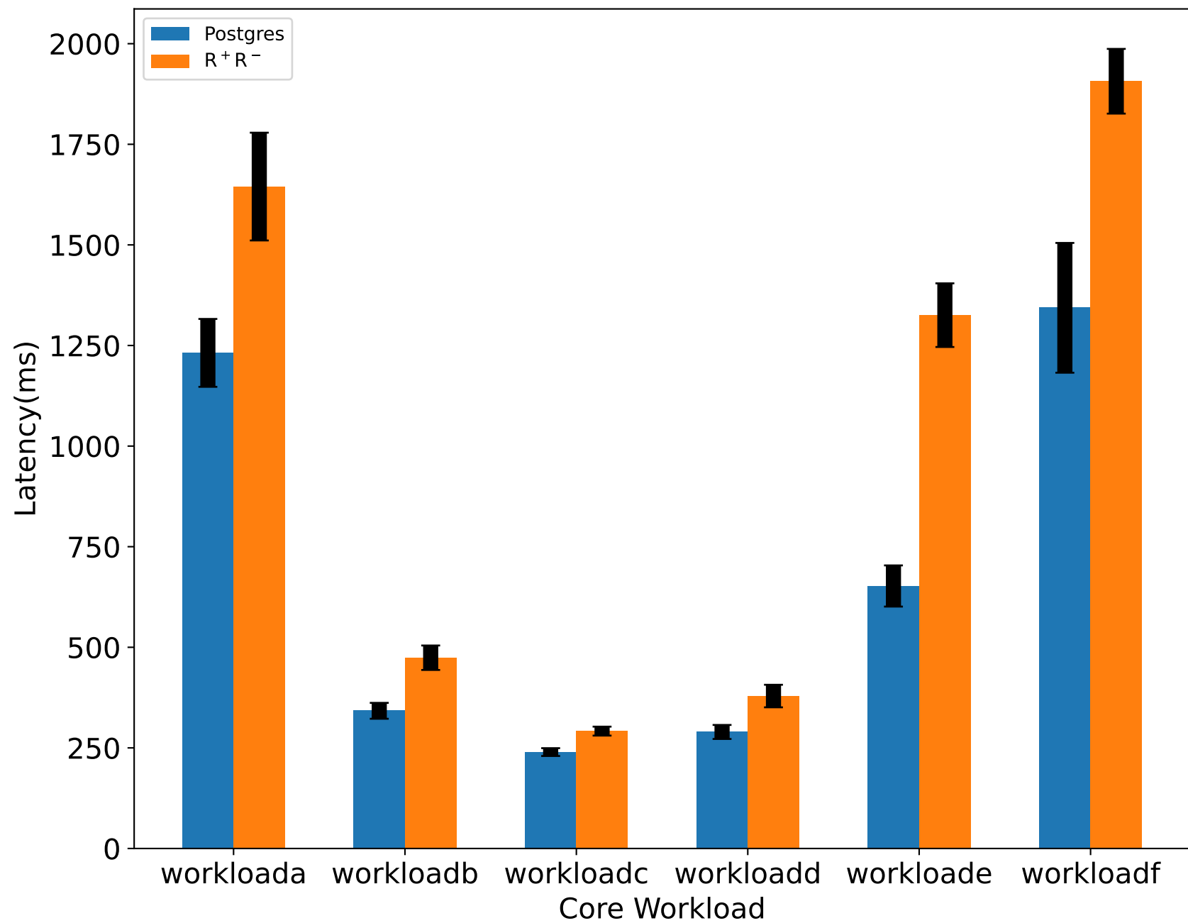
YCSB Benchmark 1M rows
