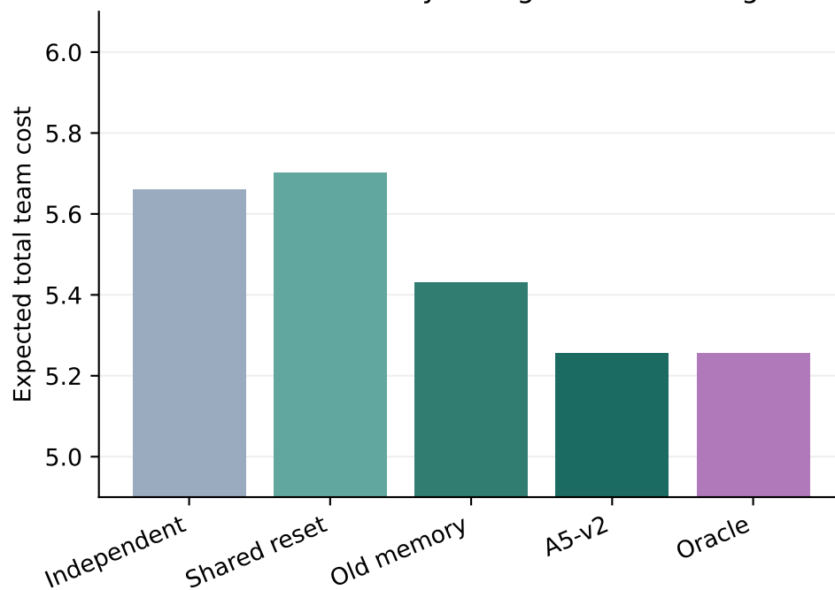
A5: finite memory changes later sensing
