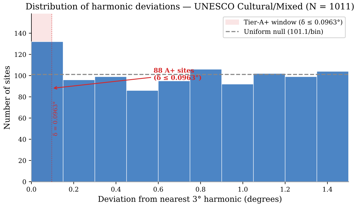
FIGURE 1 | Distribution of harmonic deviations for the full UNESCO corpus. The excess of sites within the Tier-A+ window ( \delta \leq 0.0963^\circ , shaded) above the uniform null (dashed line) establishes the corpus-level signal against which Tests 2 and 3 demonstrate morphological and spatial specificity.
