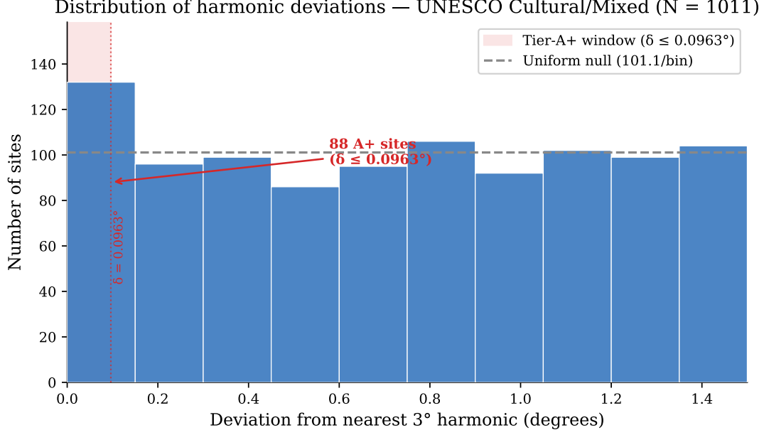
Figure 1: Distribution of harmonic deviations for the full UNESCO corpus. The excess of sites within the Tier-A+ window ( \delta \leq 0.0963 , shaded) above the uniform null (dashed line) establishes the corpus-level signal against which Tests 2 and 3 demonstrate morphological and spatial specificity.
