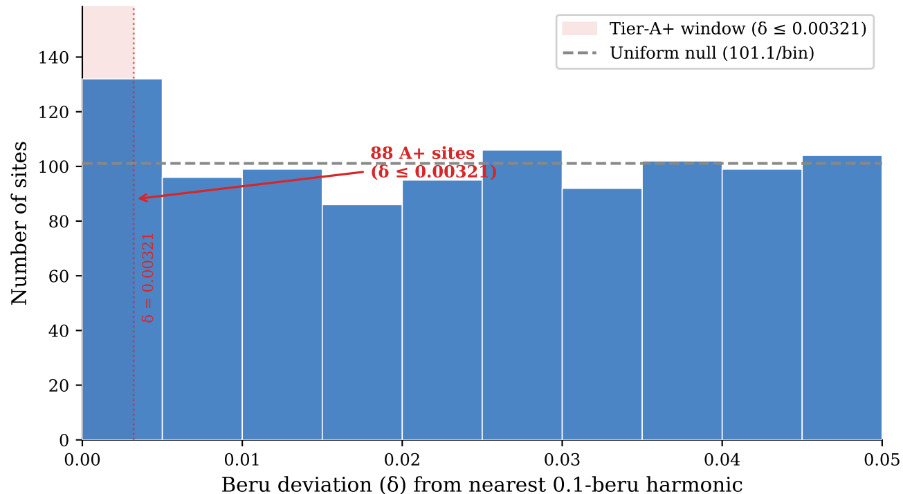
Distribution of beru deviations — UNESCO Cultural/Mixed (N = 1011)
