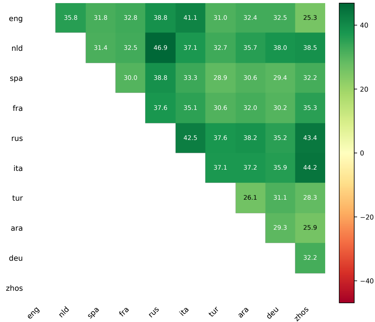
\Delta MultiBLiMP accuracy (Monolingual - Merged Bilingual, %)
