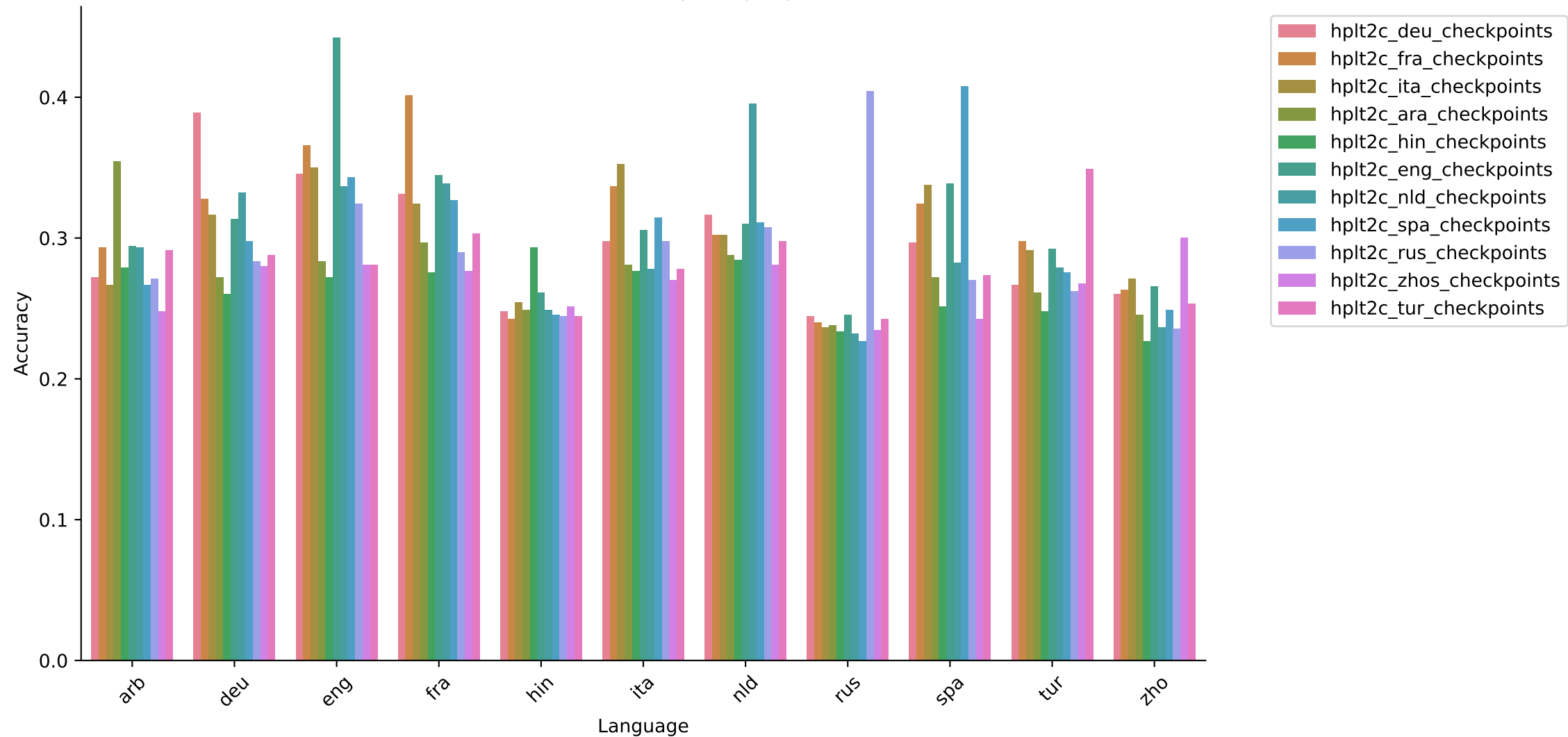
belebele Results by Language
