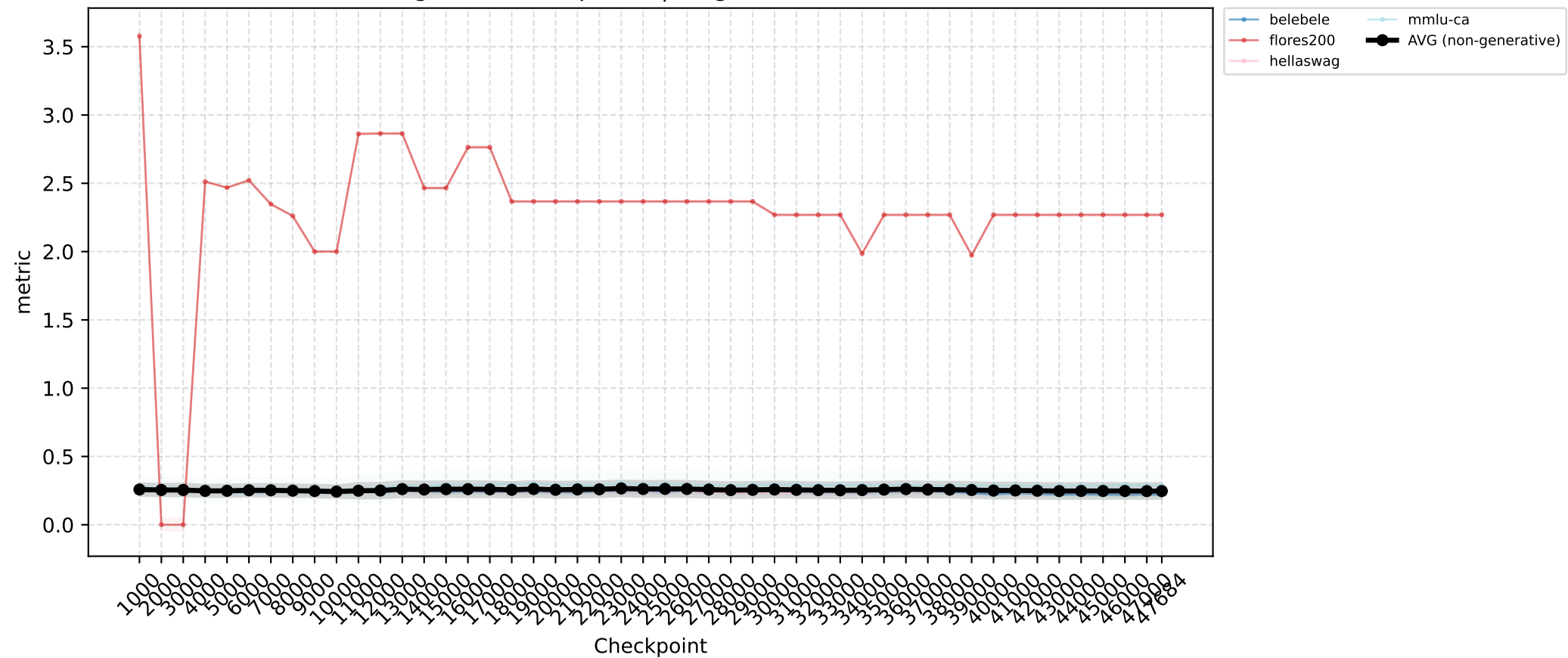
merged-10-checkpoints | lang=swe — all tasks
