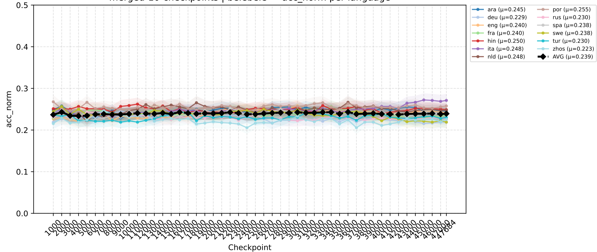
merged-10-checkpoints | belebele — acc_norm per language
