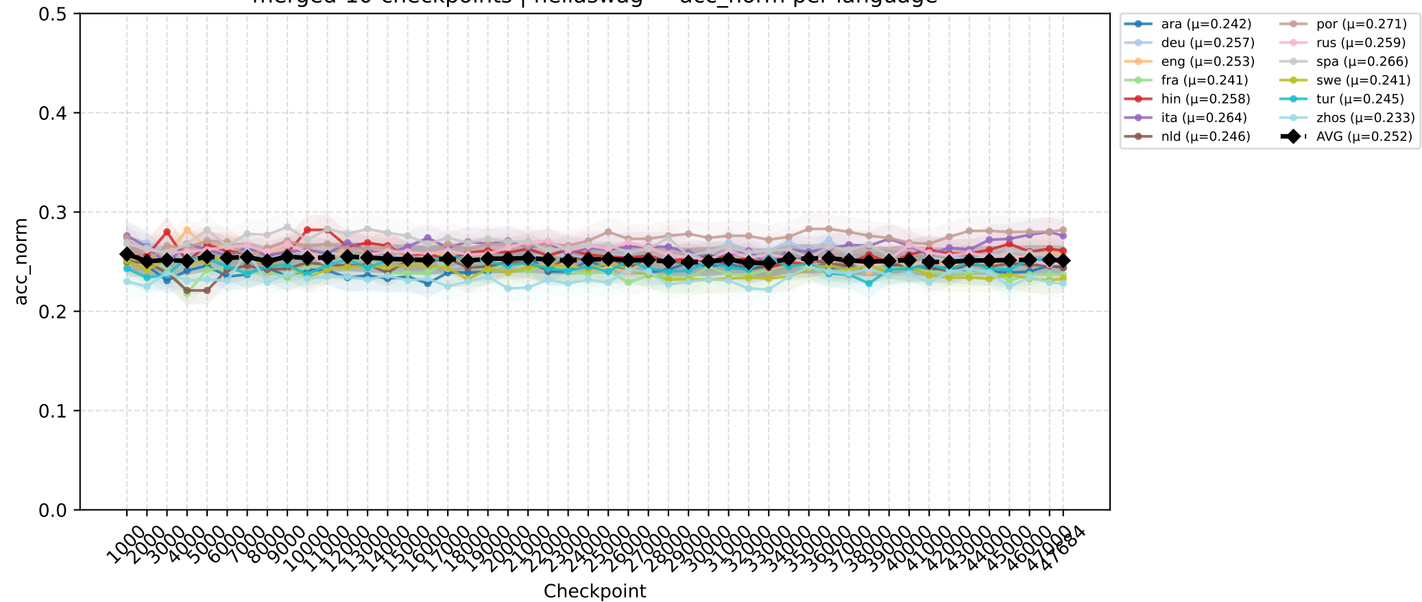
merged-10-checkpoints | hellaswag — acc_norm per language
