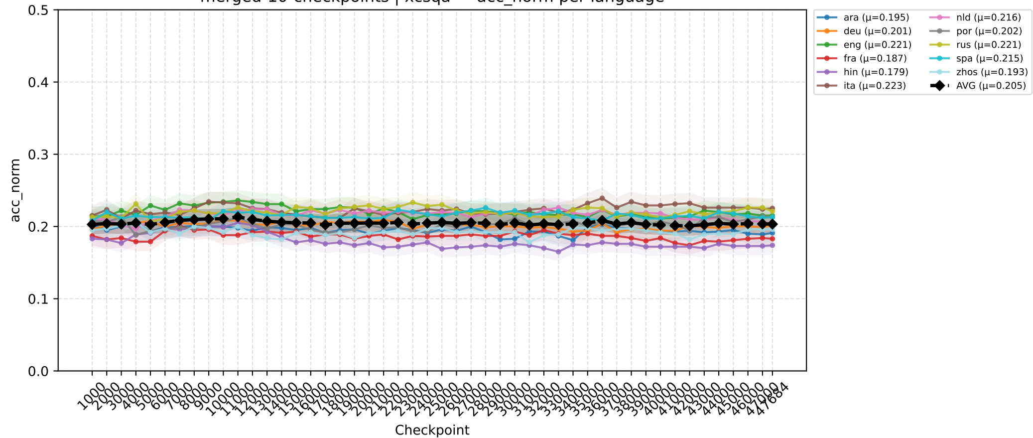
merged-10-checkpoints | xcsqa — acc_norm per language
