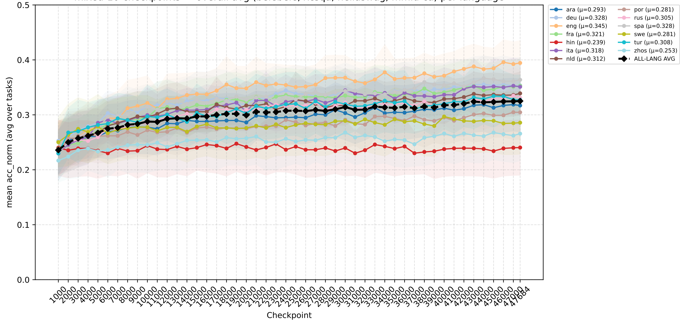
mixed-10-checkpoints — overall avg (belebele, xcsqa, hellaswag, mmlu-ca) per language
