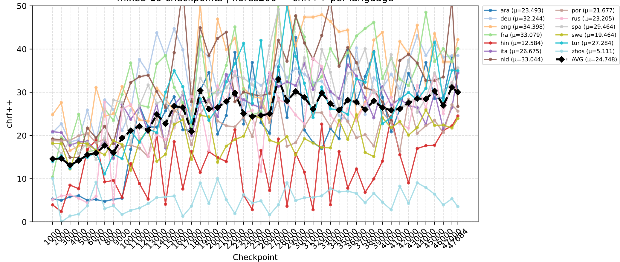
mixed-10-checkpoints | flores200 — chr++ per language
