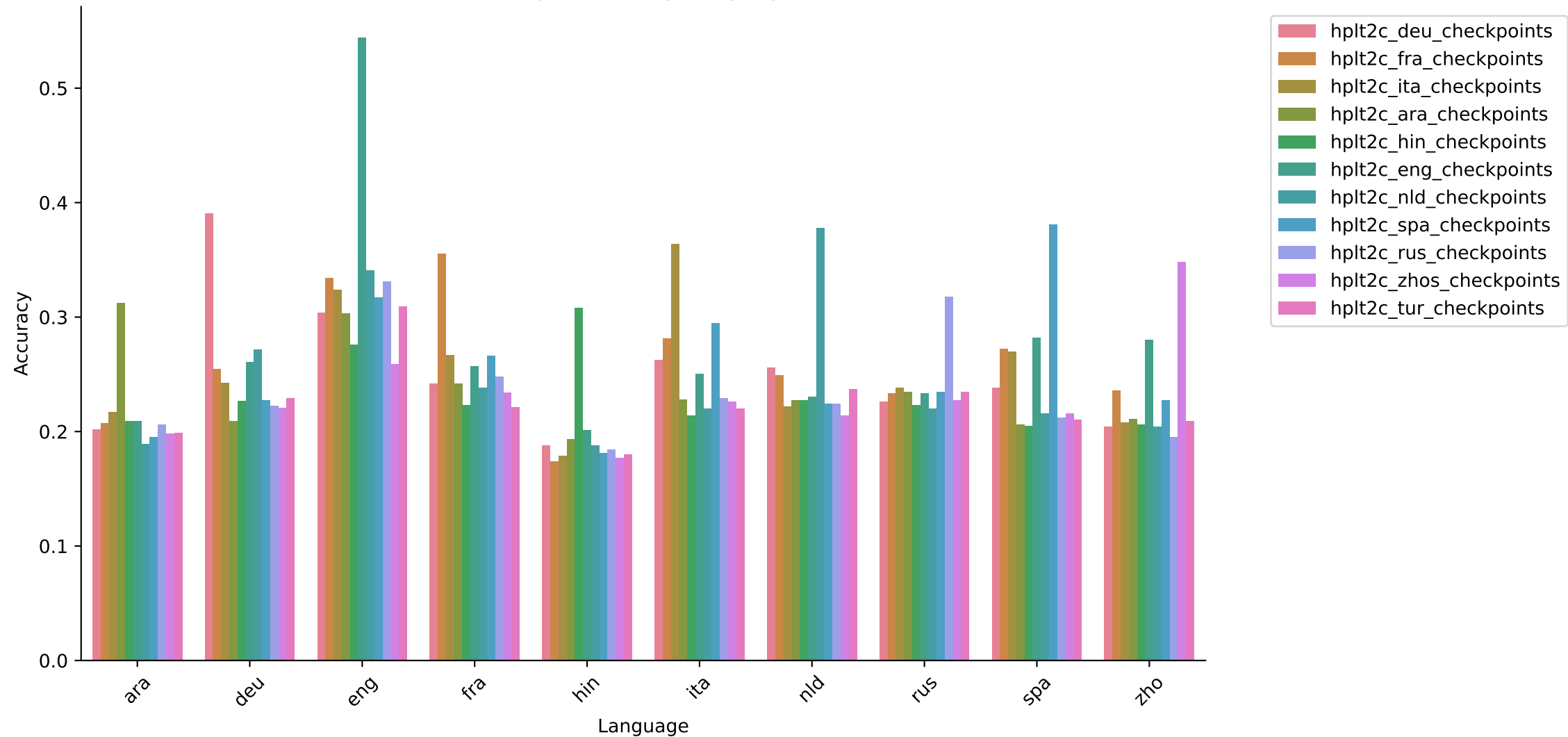
xsqa Results by Language
