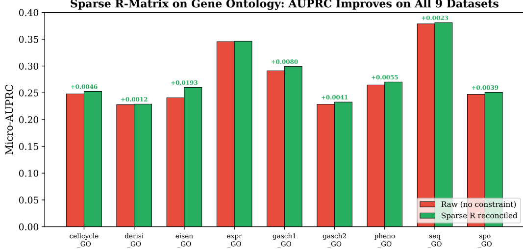
Figure 6: Sparse R-Matrix on 9 Gene Ontology datasets. AUPRC improves on all datasets (avg +0.0055).
