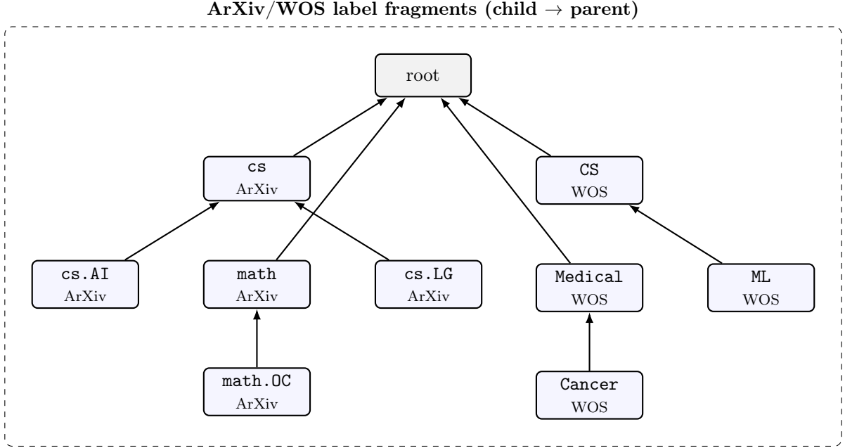
Figure 1: Hierarchy graph used by the sparse R-matrix formulation. The example uses ArXiv and WOS label fragments to mirror the datasets evaluated in the paper.
