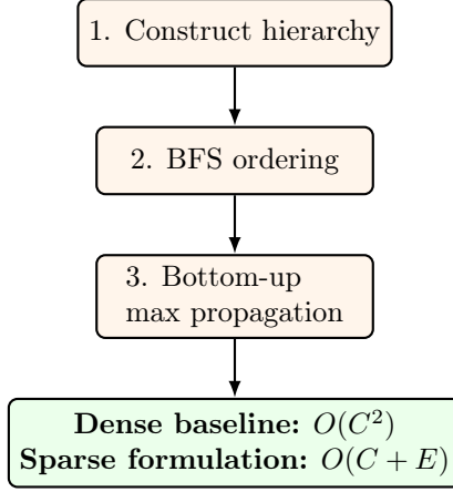
Figure 2: Sparse R-matrix flow. The sparse formulation processes the hierarchy bottom-up along the actual parent-child edges. The O(C^2) term refers only to the dense baseline; the sparse formulation uses O(C + E) memory.
