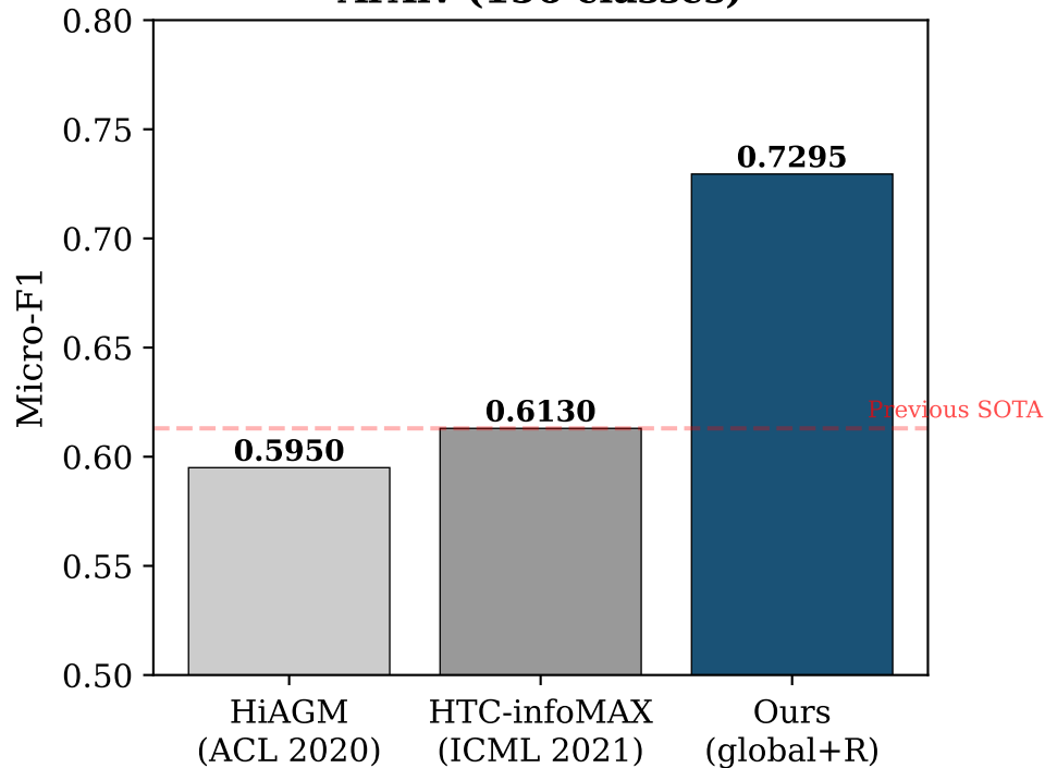
ArXiv (156 classes)
