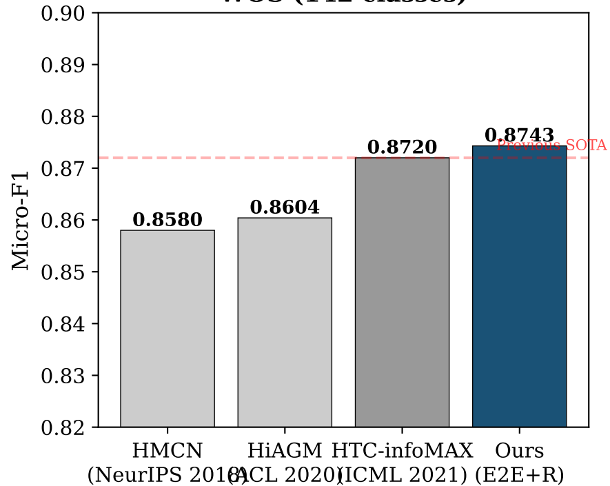
WOS (142 classes)
