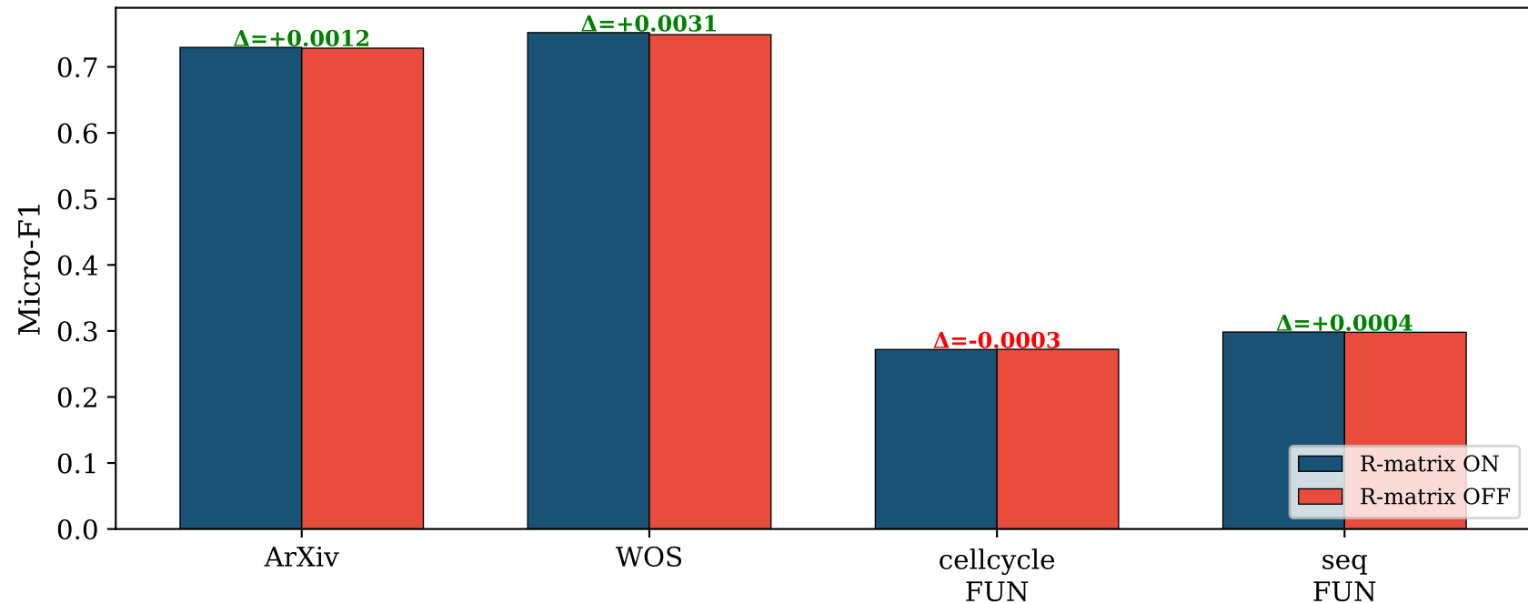
R-Matrix Ablation: Effect on Micro-F1
