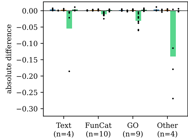
Micro-F1: change vs. plain BCE
