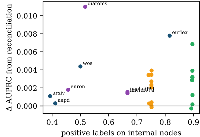
Spearman \rho = 0.08 ( p = 0.710 )
