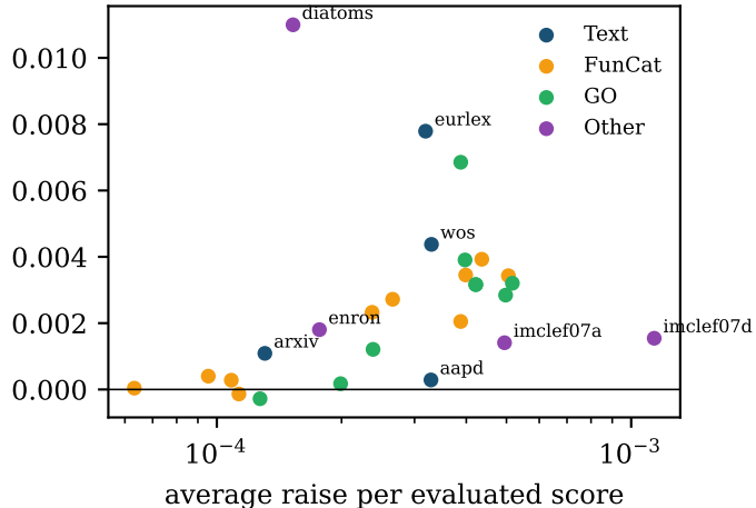
Spearman \rho = 0.54 ( p = 0.004 )
