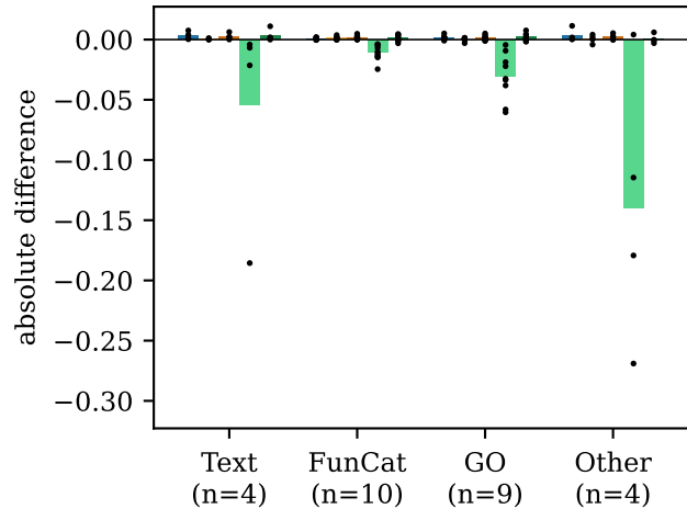
Micro-F1: change vs. plain BCE
