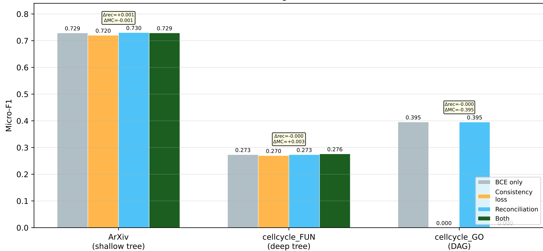
R-Matrix Ablation: Training vs Inference Contributions
